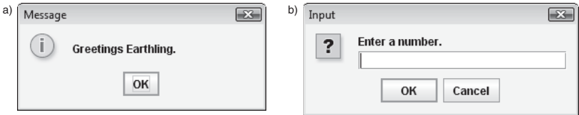
Figure 2-19 Dialog boxes
