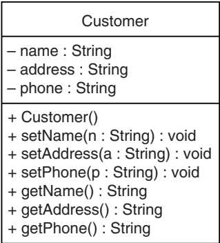
Figure 6-29 UML diagram for the Customer class
