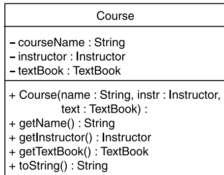
Figure 8-13 UML diagram for the Course class
