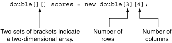
Figure 7-19 Declaration of a two-dimensional array
