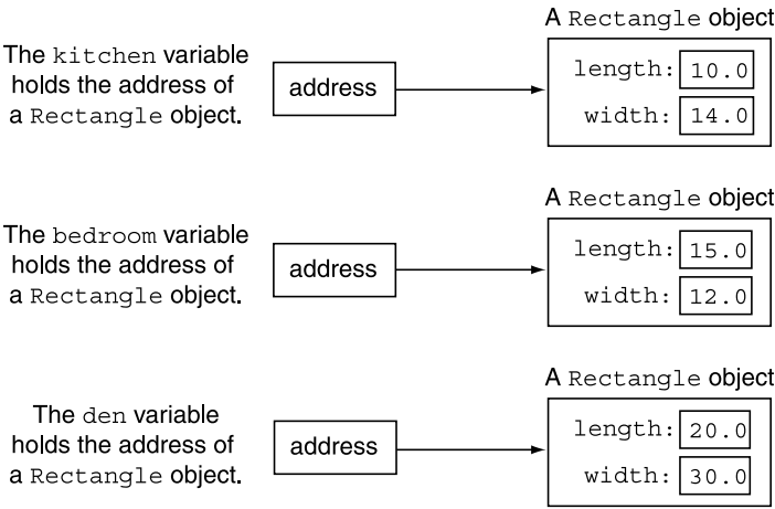
Figure 6-20 States of the objects after data has been stored in them
