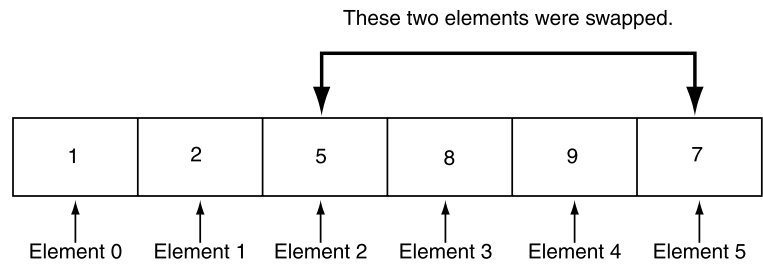
Figure 7-28 Values in array after third swap
