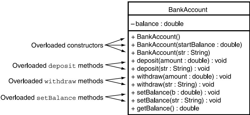
Figure 6-27 UML diagram for the BankAccount class
