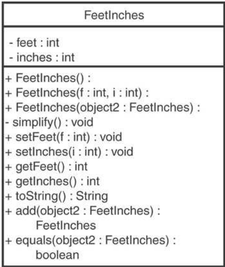
Figure CS5-1 UML diagram for the FeetInches class
