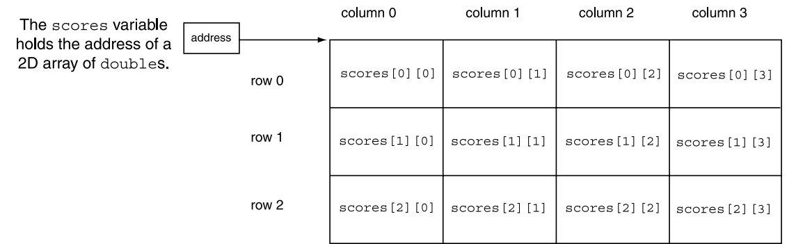
Figure 7-20 Subscripts for each element of the scores array
