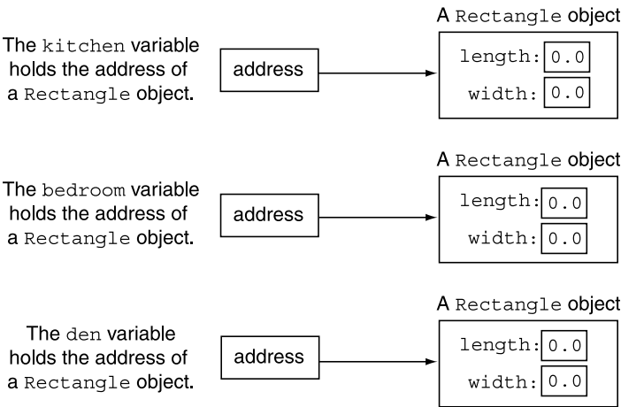
Figure 6-19 The kitchen, bedroom, and den variables reference Rectangle objects
