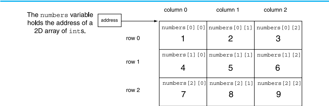
Figure 7-22 The numbers array
