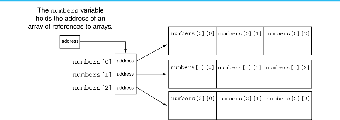
Figure 7-23 The numbers array is an array of arrays
