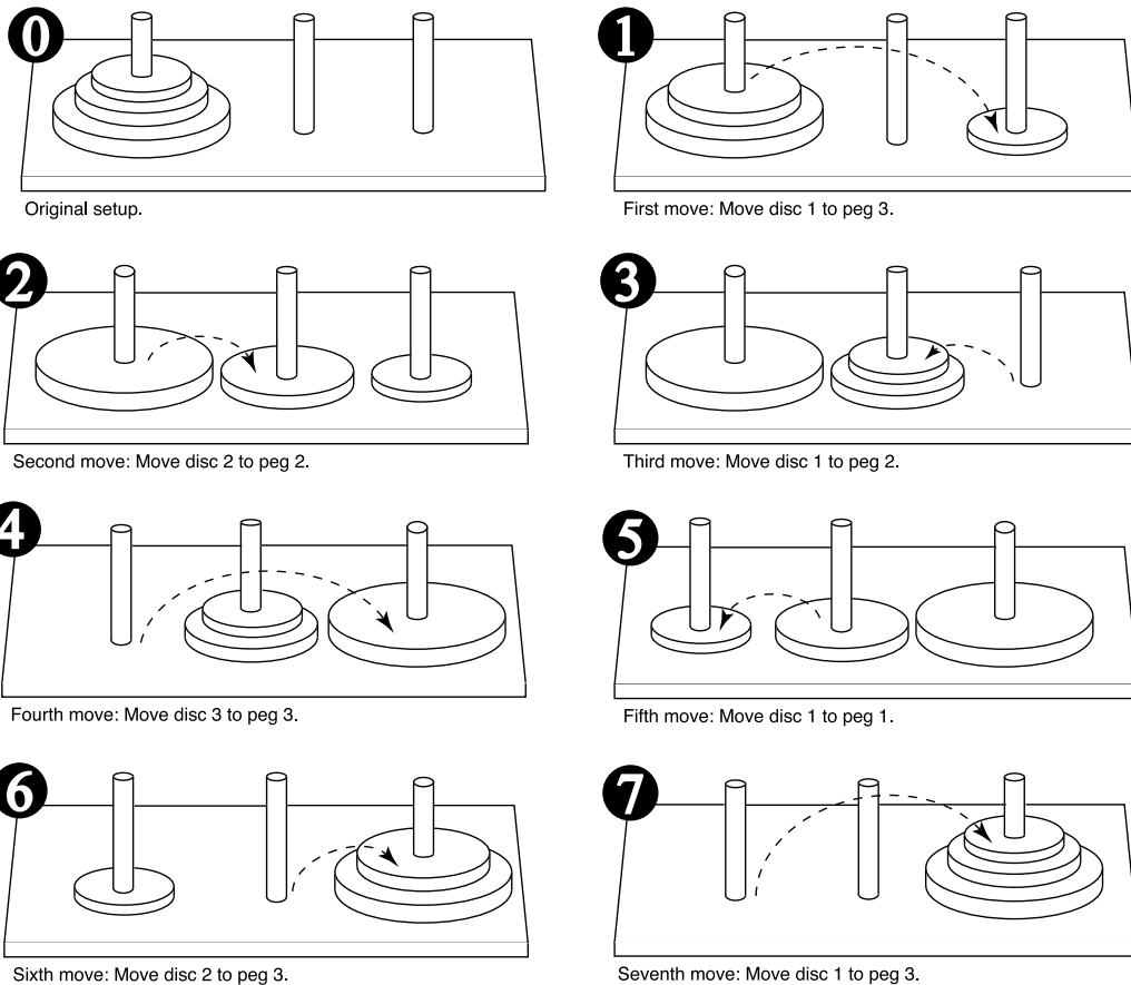
Figure 16-8 Steps for moving three pegs
