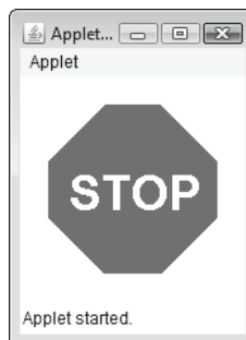
Figure 14-26 GraphicStringDemo applet
