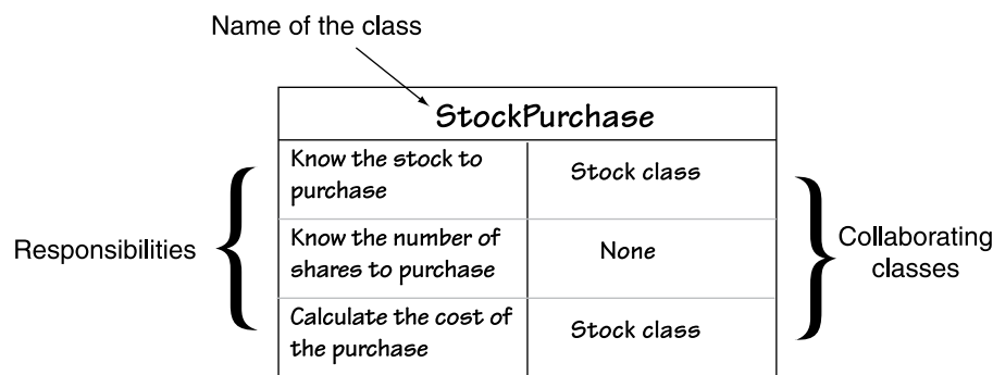
Figure 8-20 CRC card
