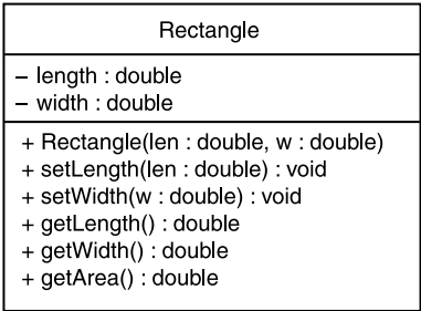
Figure 10-9 UML diagram for the Rectangle class
