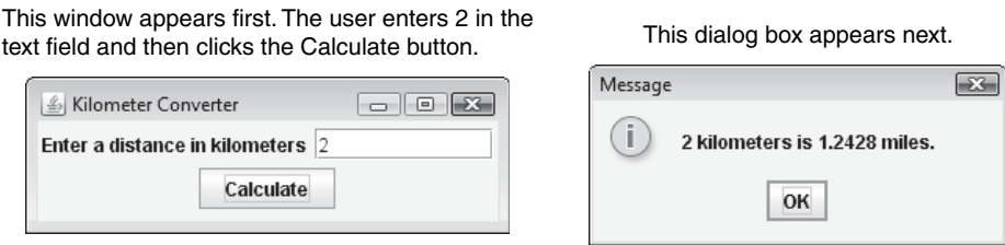
Figure 12-10 Windows displayed by the KiloConverter class (Oracle Corporate Counsel)
